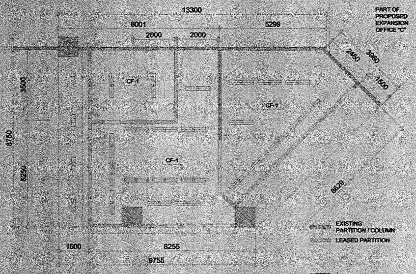
OFFICE "B" (EXISTING) AR REFLECTED CEILING PLAN SCALE: 1:50M
